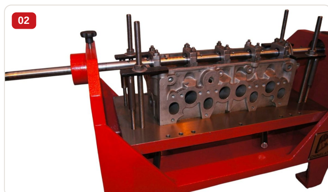
Detail — Multi-cylinder automotive cylinder head in aluminum secured in clamping device for valve guide boring operation
