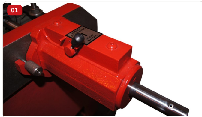
Detail — Lever for automatic advance or manual retraction with spherical handle and safety label
