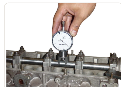
Tool height measurement with DIGIMESS dial indicator on EMC-2 boring machine
