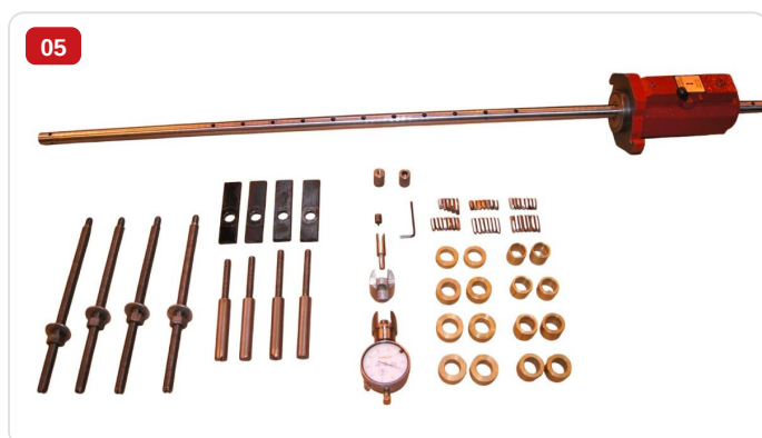
Standard accessory — Complete EMC-2 boring machine kit with tool bar, 40 carbide tools, 16 bushings, dial indicator, set screws and Allen key
