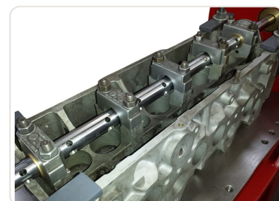
Detail view of automotive cylinder head positioned on EMC-2 boring machine showing valve train and lifter guides
