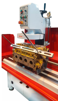
Optional accessory — DB-30/45 degrees Cradle for "V" blocks - image 01
