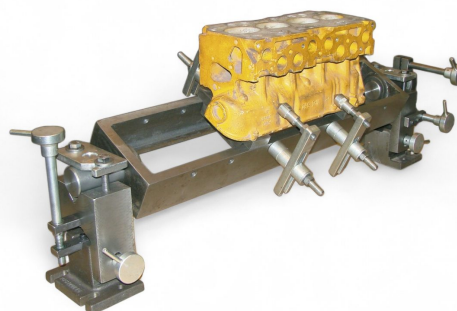
Optional accessory — American-style device for V-blocks and cylinder heads with adjustable clamping system
