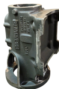
Detail — 2.051148.30 - 54 kg
