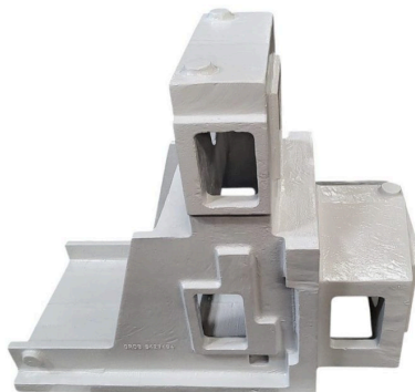
Detail — 5427493 - 484 kg
