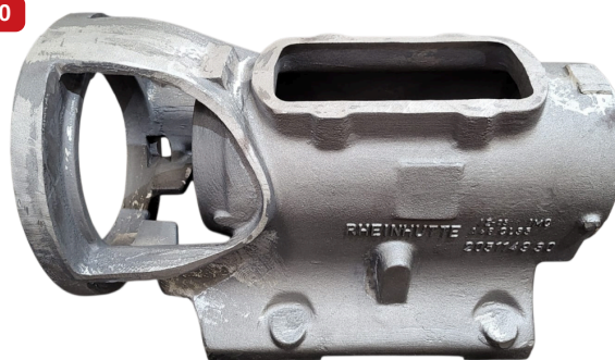
Detalle — 2.051149.30 - 140 kg
