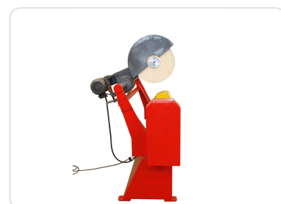
PV-1500 Chinelatto crankshaft polisher with Ø20 inch (Ø500mm) polishing disc and 3hp motor for grinding
