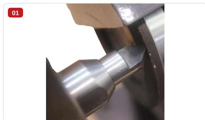
Detail — Sharpening - corner - Milling machine
