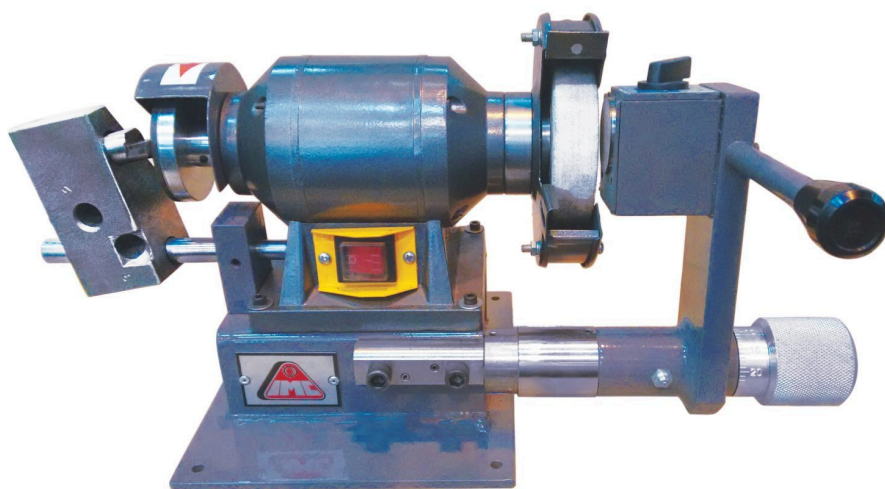
Sharpening - angle of attack - Column Boring Machine
