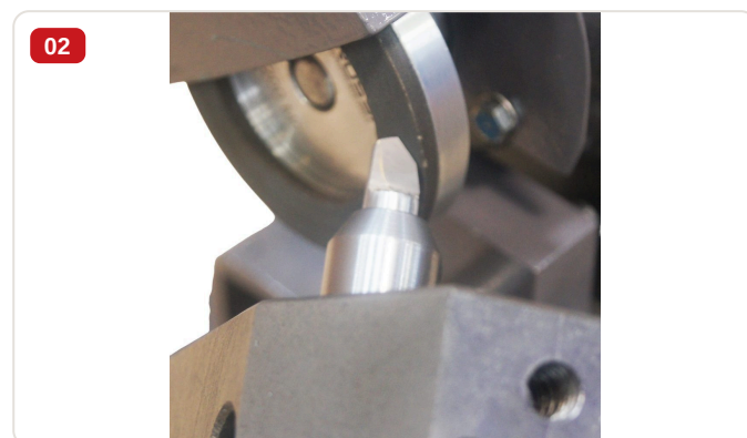
Detail — Sharpening - Tools angle 45° - general
