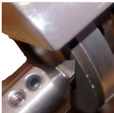
Detail — Sharpening - corner - Portable boring machine - Line boring machine
