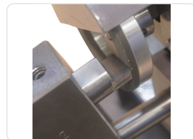
Sharpening - front angle - Column Boring Machine
