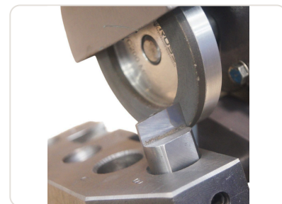
Sharpening - angle of attack - Column Boring Machine
