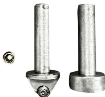
Optional accessory — Hard pre-chamber
