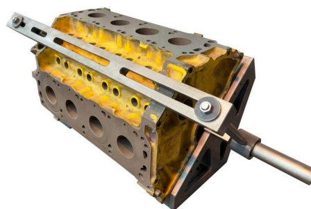
Optional accessory — Image 02 - DB-30°/45° Cradle for "V" blocks
