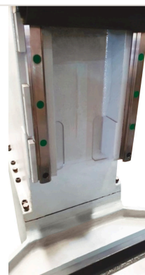
Detail — Linear guide on the column
