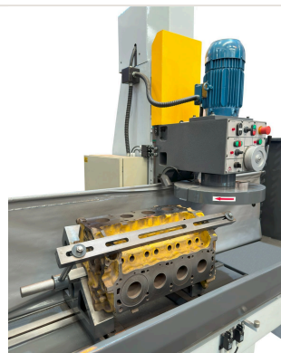
Optional accessory — Image 01 - DB-30°/45° Cradle for "V" blocks
