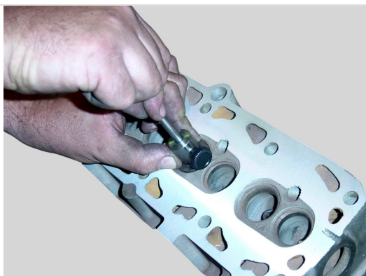
Detail — Micrometer measurement of aluminum cylinder head during resurfacing operation on RV-2 grinder
