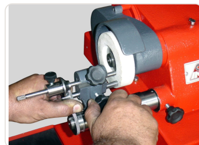
Standard accessory — Micrometric adjustment device for valve stem grinding on RV-2 valve grinder
