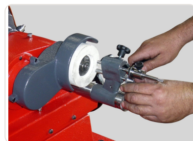
Standard accessory — Operation of RV-2 Chinelatto valve grinder with valve adjustment in collet holder
