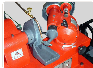
Standard accessory — RV-2 grinder head with dual grinding wheels for valves and pneumatic clamping system
