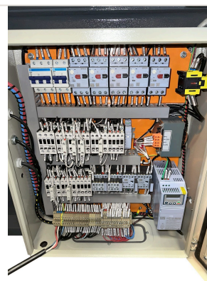
Detail — Internal electrical panel of the RVC-1000HVP with WEG MPW18 circuit breakers, contactors, terminal blocks and WEG CFW300 frequency inverter, operating at 220V three-phase
