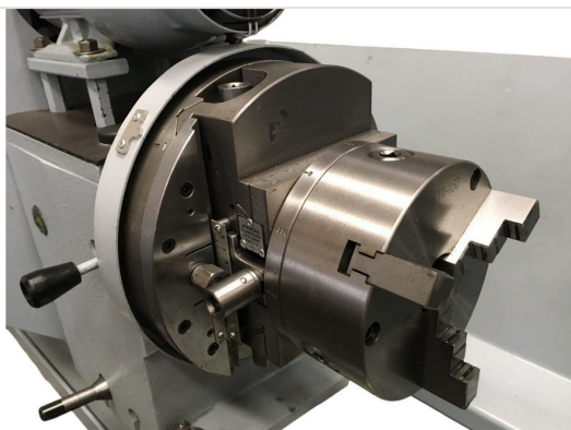
Standard accessory — Crossed Chucks with 3 jaws in cast iron for crankshaft fixation on RVC-1000M grinder
