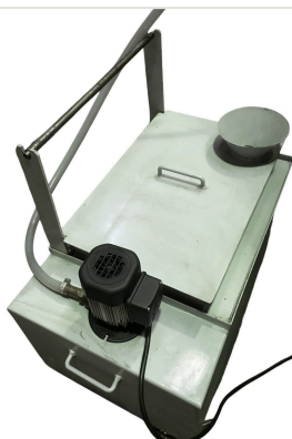
Standard accessory — Coolant reservoir with 21 gallon (80 liter) capacity and circulation pump for RVC-1000M grinder
