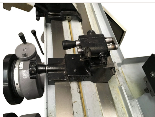
Standard accessory — Dressing device with metallic rollers for grinding wheel conditioning on RVC-1000M grinder
