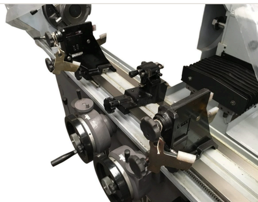
Standard accessory — Support steadies and dresser in cast iron mounted on RVC-1000M crankshaft grinding machine
