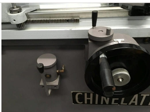
Standard accessory — Guideway lubrication pump with metal reservoir and piping system for RVC-1000M grinder
