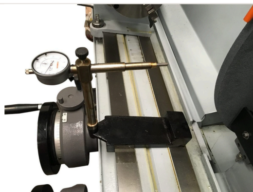
Standard accessory — Centralizing device with dial indicator for crankshaft centering on RVC-1000M grinder
