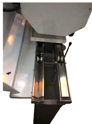
Detail — Lubrication rollers for bed ways in cast iron of RVC-1000M Chinelatto grinder
