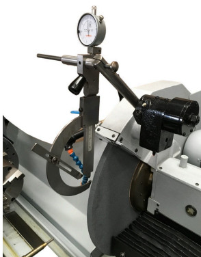
Standard accessory — Continuous measurement device (plunge) with dial indicator for dimensional control on RVC-1000M grinder
