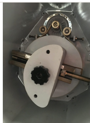
Detail — Left headstock drive system with pulleys and adjustment handwheel of RVC-1000M grinder
