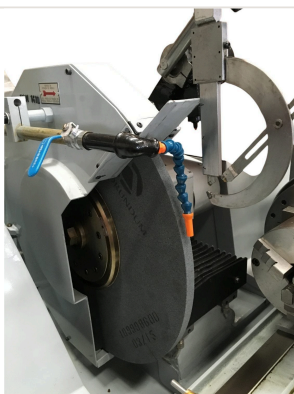
Detail — Detail of grinding wheel with fluid cooling system on RVC-1000M crankshaft grinder
