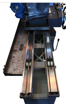
Detail — Lubrication rollers - bed with internal ribbing
