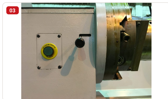
Detail — Intermittent plate rotation button on control panel of RVC-1500M crankshaft grinder
