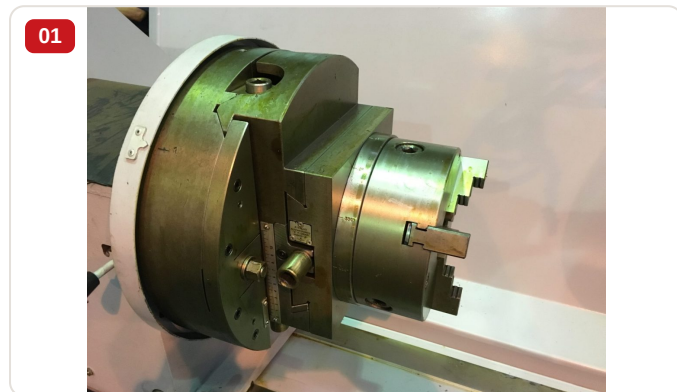
Detail — Universal chuck 8 inch with 3 jaws for crankshaft fixation in grinding machine
