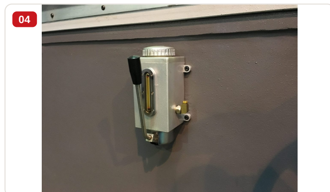
Standard accessory — Manual lubrication pump for machine bed with reservoir and level sight glass
