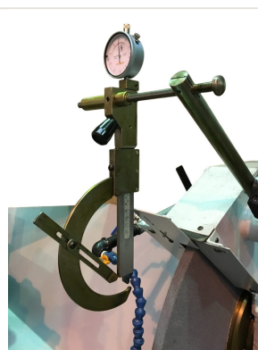
Standard accessory — Continuous measurement device with dial indicator on articulated support for dimensional control on RVC-1500M grinder
